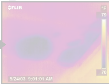
The thermogram clearly shows a leaking bedroom ceiling. The leak originated in an upstairs marble-paneled bathroom. Further IR investigation absolved the bathroom and traced the source of the leak to a clogged weep hole under the threshold of a door leading to an upstairs porch.
