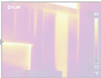
This thermogram shows where insulation is missing in the wall chamber.
